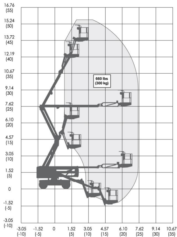
SJ45 AJ+ WORKING ENVELOPE
